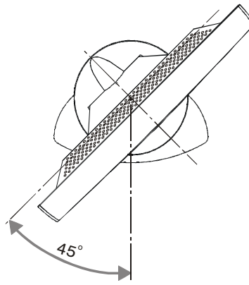
SWIVEL ANGLE-R
